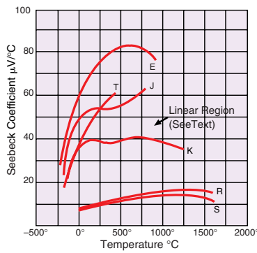
SEEBECK COEFFICIENT vs. TEMPERATURE Figure 17
